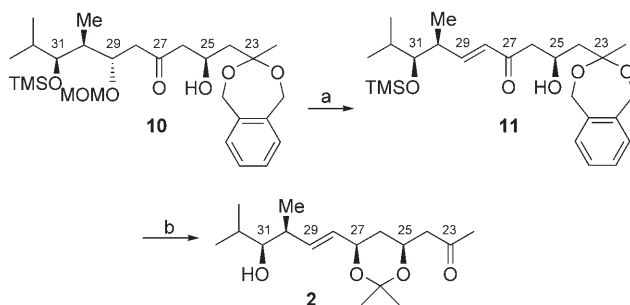
Scheme 4. Preparation of methyl ketone 2 . Reagents and conditions: a) \text{K}_2\text{CO}_3 (0.2 equiv), \text{EtOH}/\text{H}_2\text{O} 95:5 (81%, E/Z > 50:1); b) 1. \text{Et}_2\text{BOMe} , \text{NaBH}_4 ; 2. \text{FeCl}_3 , acetone, Desispheres (68%, 2 steps).
